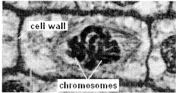
Prophase
