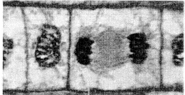
Telophase
