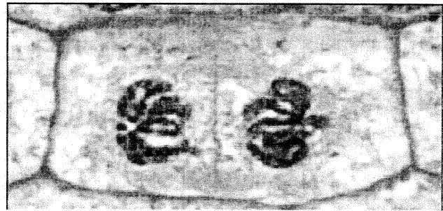
Cytokinesis
